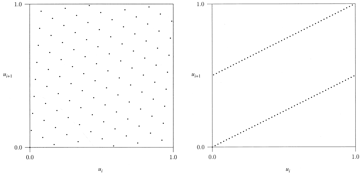
Figure 1 All pairs (u_i, u_{i+1}) for the LCGs with (n, a) = (101, 12) (left side) and (n, a) = (101, 51) (right side)
