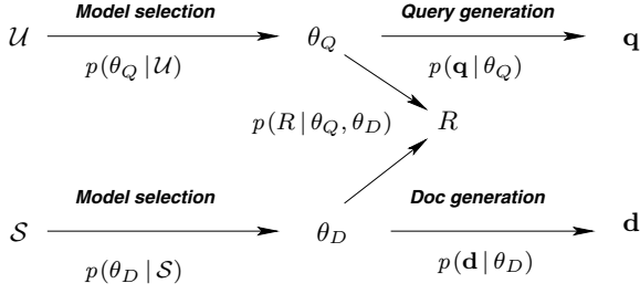
Figure 1: Generative models for queries, documents, and relevance.
