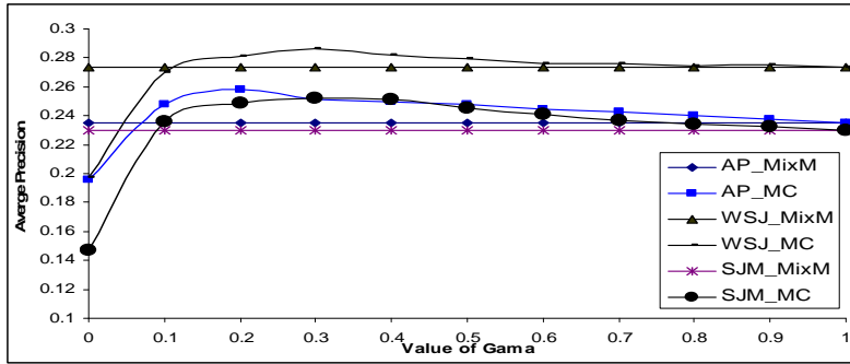
Figure 2: Sensitivity of \gamma for MC performance
