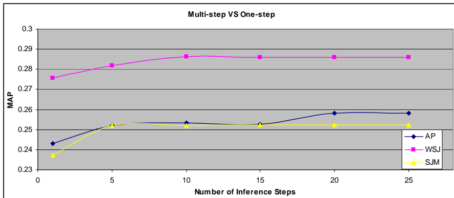
Figure 1: One-step QE Vs Multi-step MC-QE
