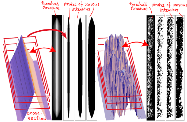
Fig. 4. Typical stroke threshold structure for etching (left) and pencil (right). We show various tonal effects conveyed by single stroke structures. The key idea is to truncate the threshold structure at a different height depending on the target tone.
