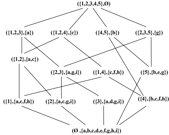
Figure 6-c. Galois lattice for relation R.
