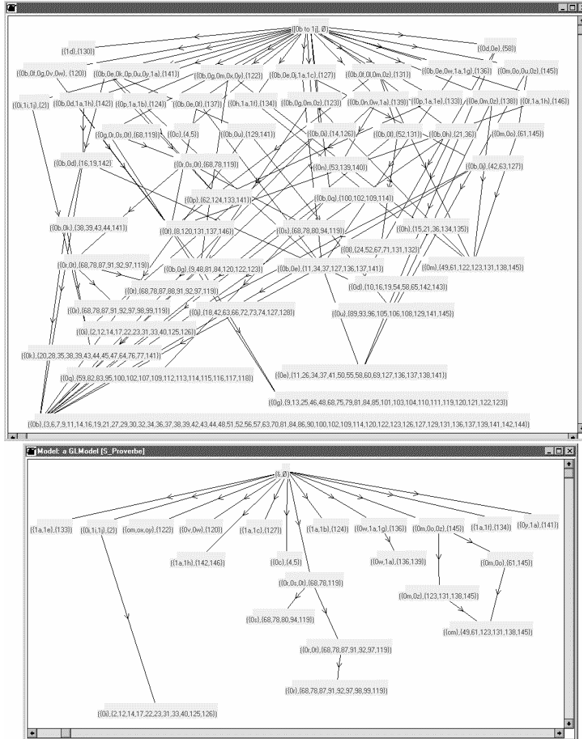
Figure 11. An overview of Galois lattice before and after removing the undesirable data for the Proverbe application
