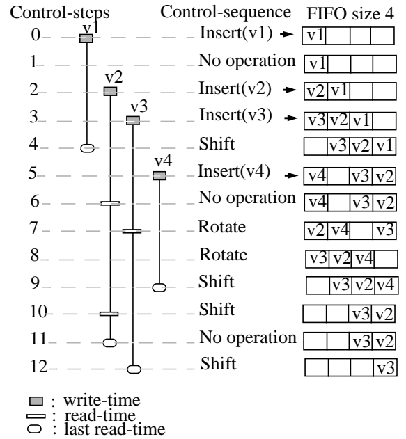
Figure 1. Illustration of the functioning of the circular FIFO
