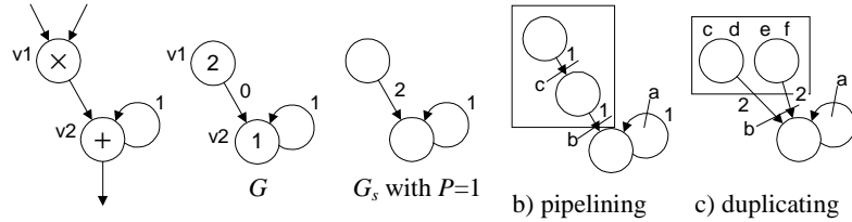
Fig. 7. Scalar product example
