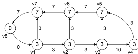
Fig. 3. Schedule graph G_s with P = 10 .
