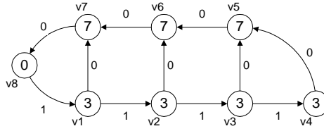
Fig. 1. A simple correlator circuit.
