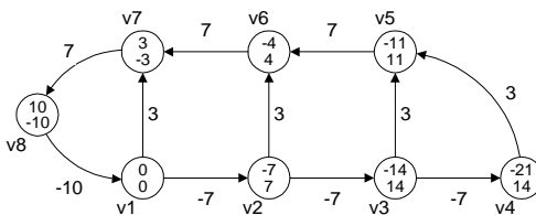
Fig. 2. G_l with the longest paths from/to v_1 in the vertices.
