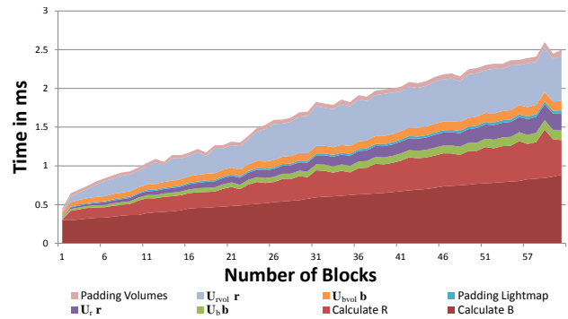
Figure 10: Average performance taken from many random mazes.
