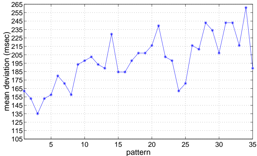
Mean deviation errors from Experiment 1 of Povel and Essens (1985)
