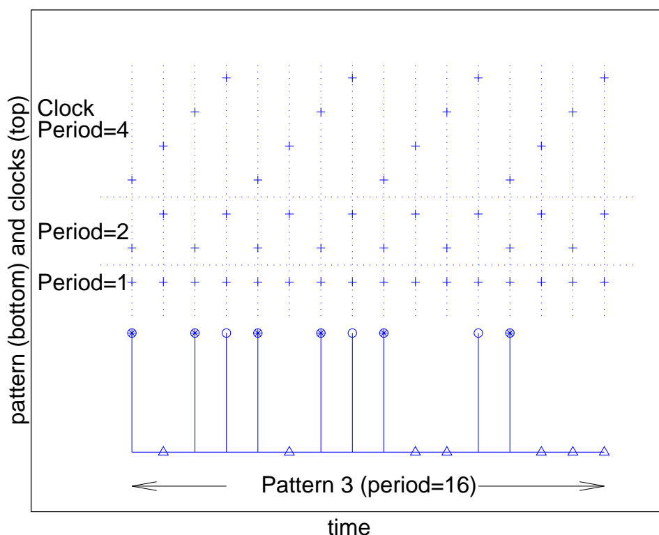
Figure 2: On the top, all seven clocks for Pattern 3 from Experiment 1 are shown as crosses. On the bottom, the pattern with accents is shown. Rests are shown as triangles, unaccented onsets as raised unfilled circles, and accented onsets as raised filled circles. Accents are assigned using the algorithm from Povel and Okkerman (1981). The horizontal axis denotes discrete time with base IOI undefined.
