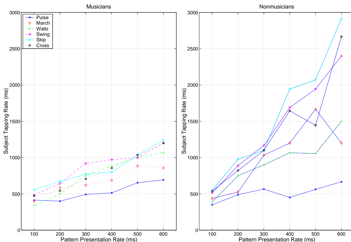
Figure 4: Data from McAuley and Semple (1999). Musicians (left) versus non-musicians (right) tapping rates. The y-axis shows the mean rate of tapping while the the x-axis shows the pattern presentation rate. Notice that musicians show a stronger tendency to tap at near 600ms regardless of presentation rate. This requires the ability to find downbeat assignments at multiple levels of the metrical hierarchy.
