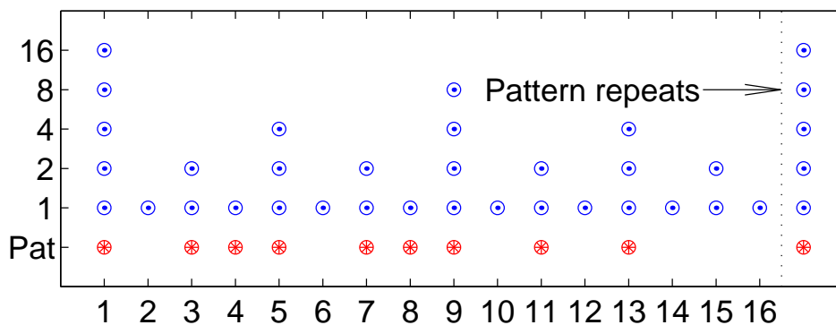
Figure 1: One candidate metrical hierarchy for a rhythmical pattern. The pattern, at the bottom, repeats every 16 time units. Progressively higher levels in the hierarchy are numbered on the vertical axis. Relatively strong events occur when many levels are aligned, such as at note 9. Alternately, events in the input that coincide with few levels in the hierarchy are relatively weak, such as at note 6.
