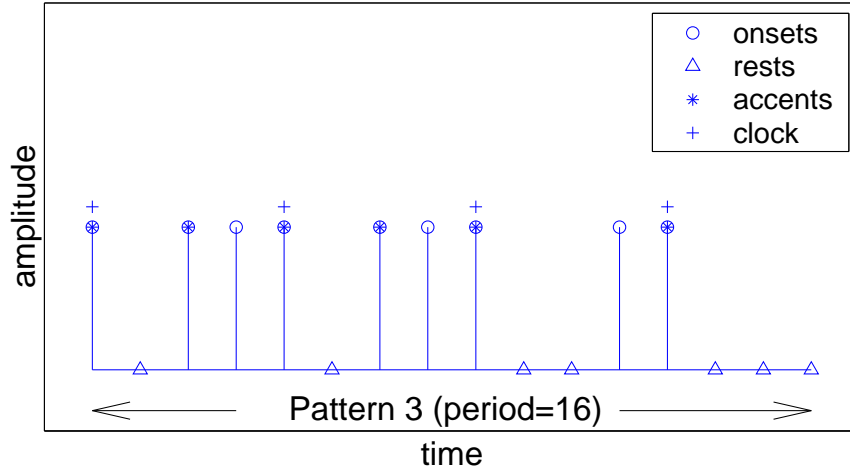
Figure 3: The best clock as predicted by all four competing models for Pattern 3 from Experiment 1 of Povel & Essens (1985). The best clock is shown above the pattern as a series of crosses. Accents are from Povel and Okkerman (1981).
