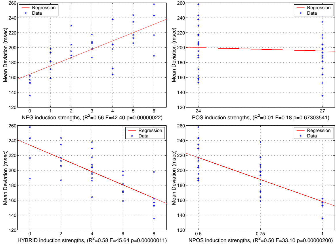
Figure 6: The regression results are shown for all four clock models. To form the regression line, the data from Experiment 1 of Povel & Essens (1985) were regressed onto the clock strengths. The reversed slope for the NEG model is due to the fact that a high NEG value indicates a low clock induction strength.
