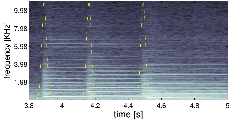
Figure 4: The magnitude plane of the STFT of a guitar recording. The sampling frequency is 22050 Hz, the window width is 30 ms and the overlapping factor is 0.9. The dashed line reveals the labeled onsets positions.
