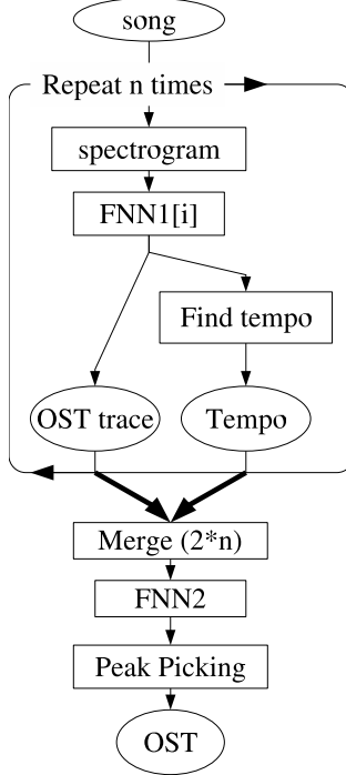
Figure 3: MULTI-NET flow chart. The SINGLE-NET variant is repeated multiple times with different hyperparameters. A tempo detection algorithm is run on each of the resulting feed-forward neural network (FNN) outputs. The SINGLE-NET outputs and the tempo detection outputs are then combined using a second neural network.
