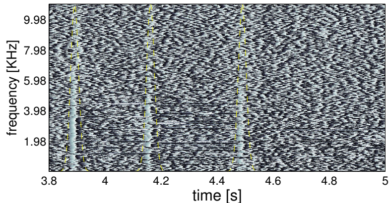
Figure 8: The phase plane of the STFT of Figure 4, transformed according to Equation 6. The dashed line represents the labeled onsets positions.
