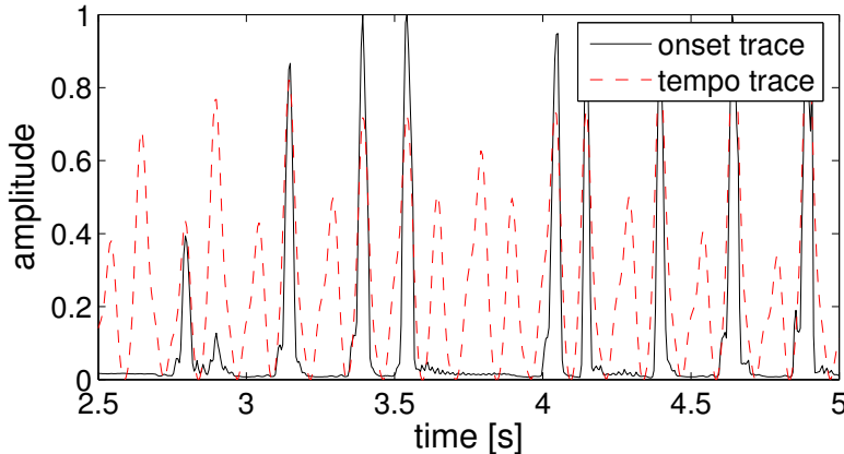
Figure 11: The onset trace shows the merged output of the neural networks as in Figure 10. The tempo trace shows the cross-correlation of the onset trace with it’s own autocorrelation.
