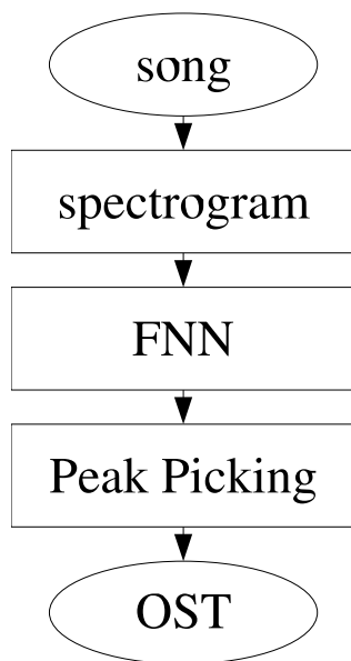
Figure 2: SINGLE-NET flow chart. This simpler variant of our algorithm is comprised of a time-space transform (spectrogram) which is in turn treated with a feed-forward neural network (FNN). The resulting trace is fed into a peak-picking algorithm to find onset times (OST).
