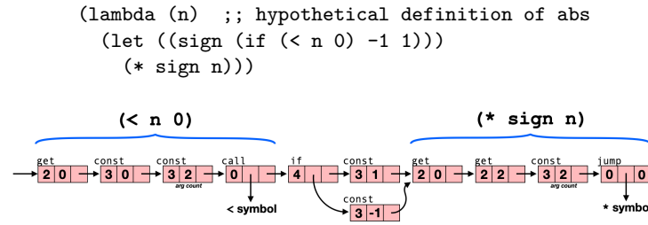
Fig. 1. RVM code represented as ribs. The RVM code corresponds to the body of the lambda-expression.
