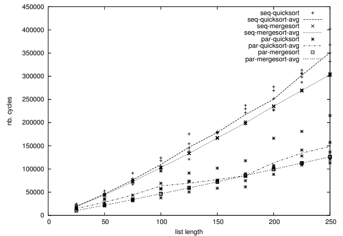
Figure 5. Sequential and parallel mergesort vs. quicksort, number of cycles as a function of list length
