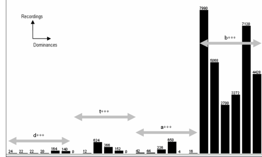
Fig. 4. Dominance Values Repartition.
