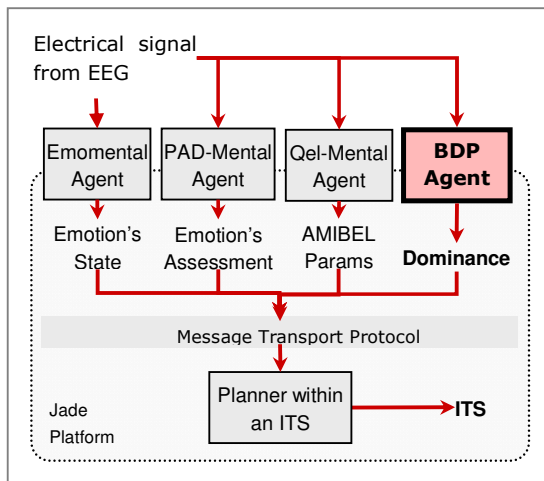
Fig. 6. Extended Architecture of the Multi-Agent Brain-Sensitive System.
