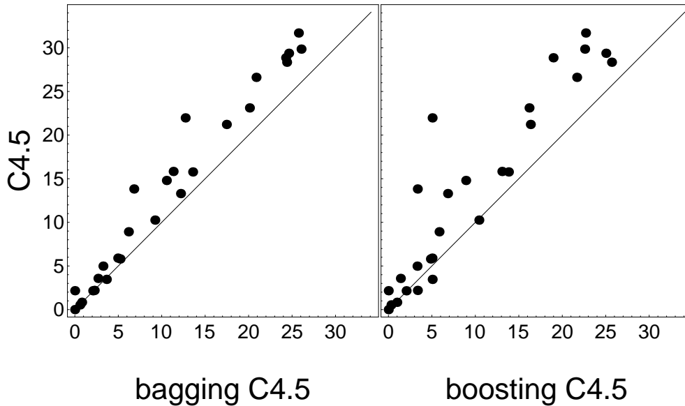
Figure 2: Comparison of C4.5 versus bagging C4.5 and boosting C4.5 on a set of 27 benchmark problems as reported by Freund and Schapire [18]. Each point in each scatter plot shows the test error rate of the two competing algorithms on a single benchmark. The y -coordinate of each point gives the test error rate (in percent) of C4.5 on the given benchmark, and the x -coordinate gives the error rate of bagging (left plot) or boosting (right plot). All error rates have been averaged over multiple runs.
