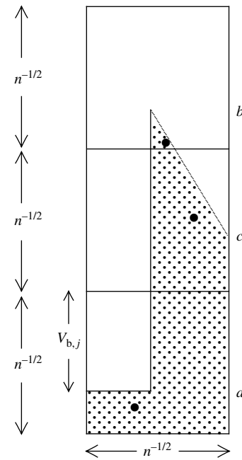
Figure A.1. Illustration of the proof of Lemma 2.
