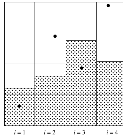
Figure A.2. An example of a histogram H_{j,z} for n = 4 .
