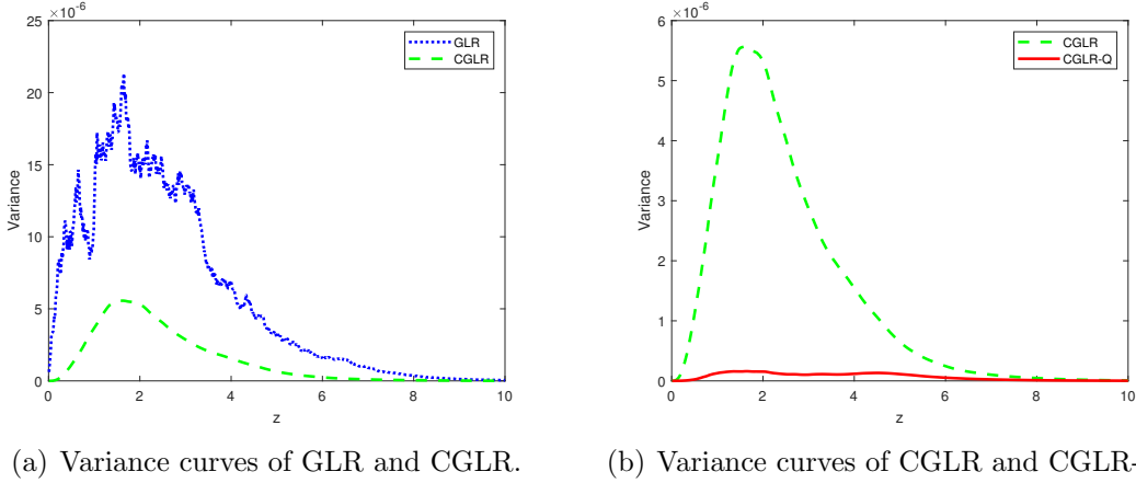
Figure 2: Variance comparison between GLR, CGLR, and CGLR-Q estimators for estimating the density of g(U; \theta) in the example of Section 5.1. We take the average and variance of 100 independent replicates of a RQMC estimate with scrambled Sobol' point set with n = 2^{13} points and of the average of 2^{13} independent simulations, respectively.
