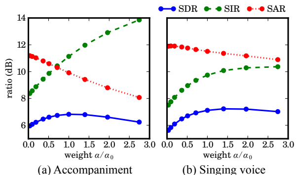
Fig. 3. Source separation performance trade-off on the MIR-1K test set by supervised NMF with an RNN-RBM model weighted by \alpha , where \alpha_0 maximizes the validation SDR.
