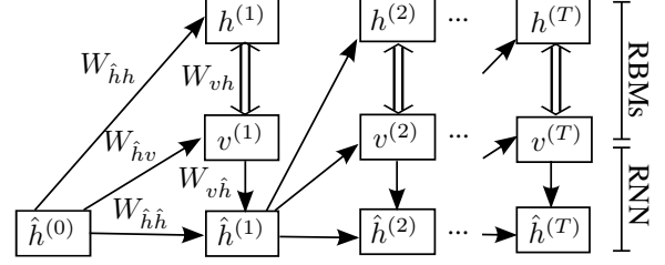
Fig. 1. Graphical structure of the RNN-RBM. Single arrows represent a deterministic function, double arrows represent the stochastic hidden-visible connections of an RBM.
