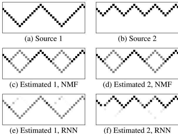
Fig. 2. Toy example: separation of sawtooth wave sources of different amplitudes (a–b) using supervised NMF with either no prior (c–d) or an RNN with the cosine distance cost (e–f).
