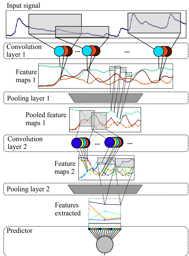
Fig. 1. Structure of an example deep ANN architecture. The architecture contains: a) a convolutional neural network (CNN) with two convolution and two pooling layers, and b) a single layer perceptron (SLP) predictor. In the illustrated example the first convolution layer process a skin conductance signal which is propagated forward through the pooling and convolution layers of the architecture. The output of the CNN provides a number of extracted (learned) features which feed the input of the SLP predictor.
