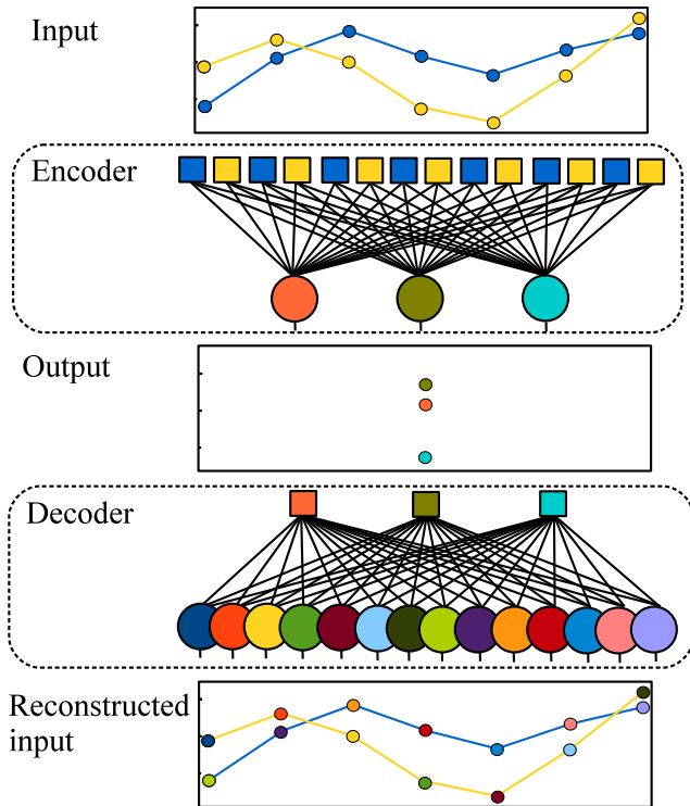
Fig. 2. Structure of an auto-encoder. The encoder generates the outputs from the input signals. During training the outputs are fed to a decoder that reconstructs the input.
