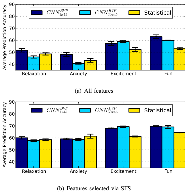
Fig. 5. Blood Volume Pulse: average accuracy of ten SLPs trained on statistical features (Statistical), and features pooled from each of the CNN topologies ( CNN_{1x45}^{BVP} and CNN_{30x45}^{BVP} ). The black bar displayed on each average value represents the standard error.
