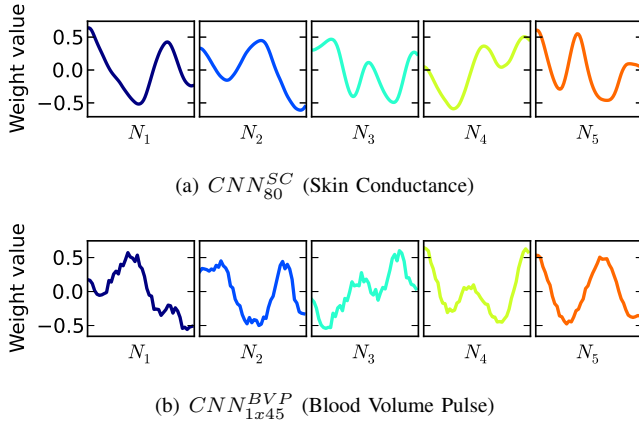
Fig. 3. Learned features of the best-performing convolutional neural networks. Lines are plotted connecting the values of consecutive connection weights for each neuron N_x .
