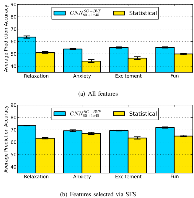
Fig. 6. Fusion of SC and BVP signals: average accuracy of ten SLPs trained on blood volume pulse and skin conductance using statistical features on the raw signal (Statistical) and features pooled from CNN_{80}^{SC} and CNN_{1x45}^{BVP} ( CNN_{80+1x45}^{SC+BVP} ). The black bar displayed on each average value represents the standard error.
