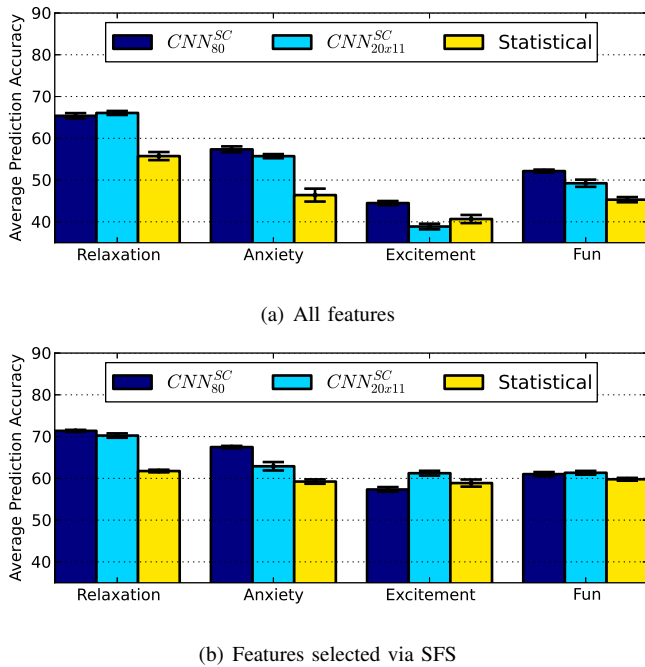
Fig. 4. Skin Conductance: average accuracy of ten SLPs trained on statistical features (Statistical), and features pooled from each of the CNN topologies ( CNN_{20 \times 11}^{SC} and CNN_{80}^{SC} ). The black bar displayed on each average value represents the standard error.
