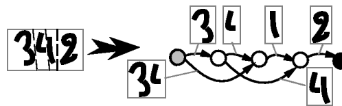
Fig. 16. Building a segmentation graph with Heuristic Over-Segmentation.
