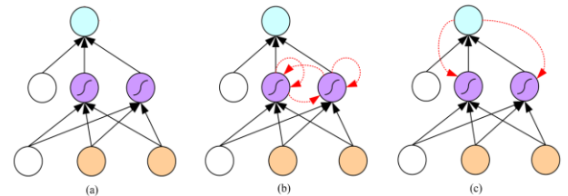
(a) Feed-forward NN; (b) Elman-RNN; (c) Jordan-RNN
