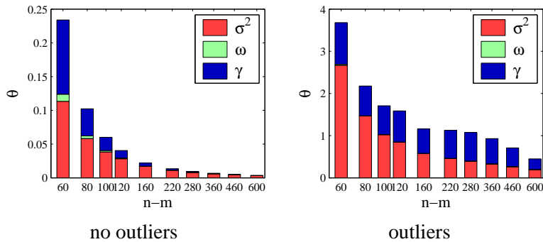
Figure 4: Bar plots of the contributions to total variance Var[CV] due to \sigma^2 , \omega and \gamma vs. the number of training examples n - m .
