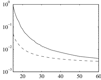
Figure 1: Estimates of the variance of \widehat{\text{EPE}}(n) vs. empirical variance of \widehat{\text{EPE}}(n) (shown by bold curve) on 100 000 experiments. The average of the variance estimators \hat{\theta}_1 (ignoring correlations, dashed curve) and \hat{\theta}_2 (taking into account correlations, dotted curve) are displayed for different training sample size n .
