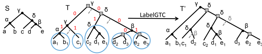
■ Figure 1 Left. A species tree S for \Sigma = \{a, b, c, d, e\} , a reconciled 0-1 edge-labelled gene tree T for \Gamma = \{a_1, b_1, c_1, c_2, d_1, d_2, d_3, e_1, e_2, e_3\} where each leaf x_i denotes a gene belonging to species x , and a covering set \mathcal{T} of subtrees for T indicated by circles around each subtree. Square nodes are duplications and circular nodes are speciations. Internal nodes are labelled according to corresponding ancestral species in S . Dotted lines are losses. Right. A supertree for \mathcal{T} of minimum reconciliation cost (cost of 5) respecting the edge labelling of T .
