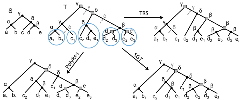
Figure 2 Top left. Species tree S for \Sigma = \{a, b, c, d, e\} , gene tree T for \Gamma = \{a_1, b_1, c_1, c_2, d_1, d_2, d_3, e_1, e_2, e_3\} with a covering set \mathcal{T} of subtrees for T as in Figure 1 (without the 0-1 labelling of edges). Bottom left. A polytomy resolution supertree for \mathcal{T} of minimum reconciliation cost (cost of 3). Bottom right. A supertree for \mathcal{T} of minimum reconciliation cost (cost of 3). Top right. A triplet respecting supertree for \mathcal{T} of minimum reconciliation cost (cost of 5). Note that the three optimal supertrees for the TRS, SGT and PolyRes problems differ from the optimal supertree for the LabelGTC problem depicted in Figure 1, because the implicit 0-1 edge-labellings differ from the one in Figure 1.
