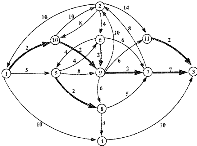
Figure 7 Network Used for the Numerical Tests
