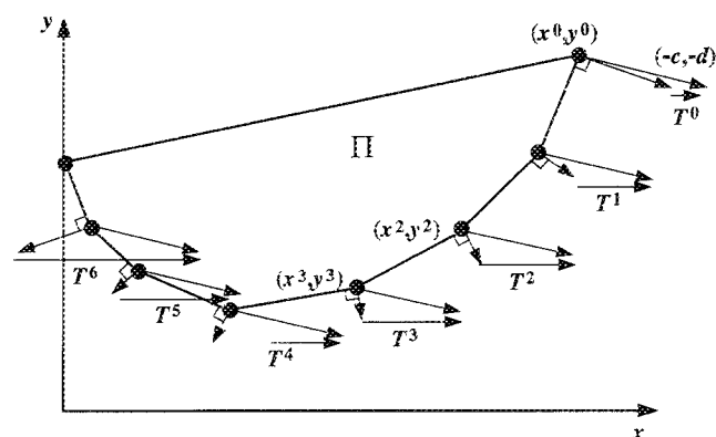
Figure 1 A Two-Dimensional Example
