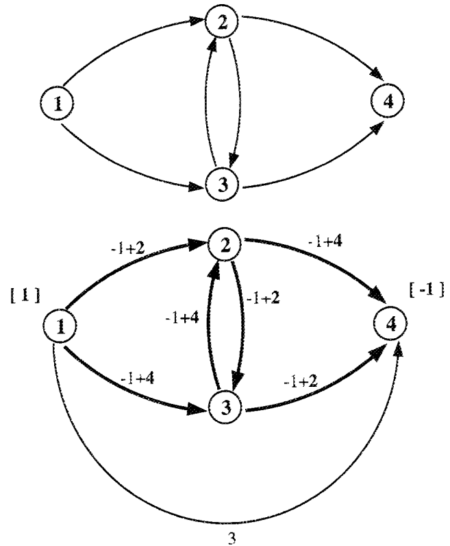
Figure 3 The Graph Transformation
