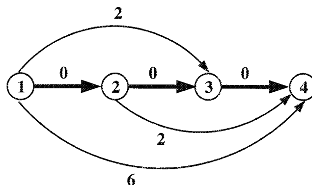
Figure 6 An Optimal Solution with a Negative Toll Value
