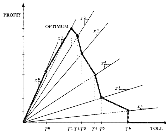
Figure 2 Upper Envelope of the Function F(x, T), y(T), T
