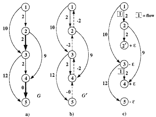
Figure 5 The Input Graph G and the Modified Graph G'
