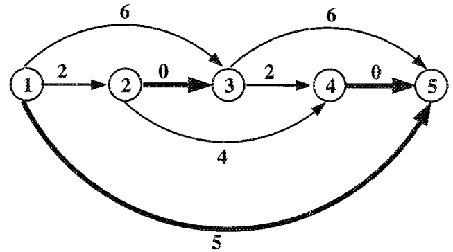
Figure 4 The Upper Bound is not Reached
