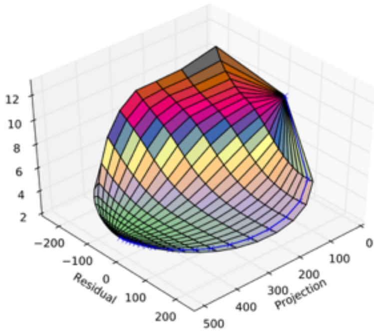
LSTM
