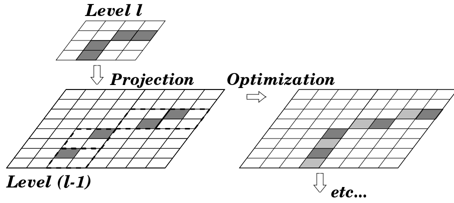
FIG. 3: “Coarse-to-fine” minimization strategy. The initial snake position for the next lower level is then obtained by keeping the descendant (among four) of each node ensuring the minimal external energy.
