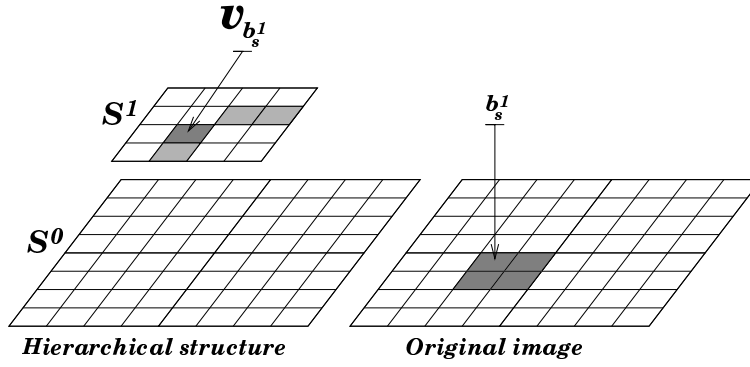
FIG. 2: Hierarchical structure ( L = 1 in this example) involved in the multiscale minimization strategy and block of pixels b_s^l associated to the node \mathbf{v}_{b_s^l} .
