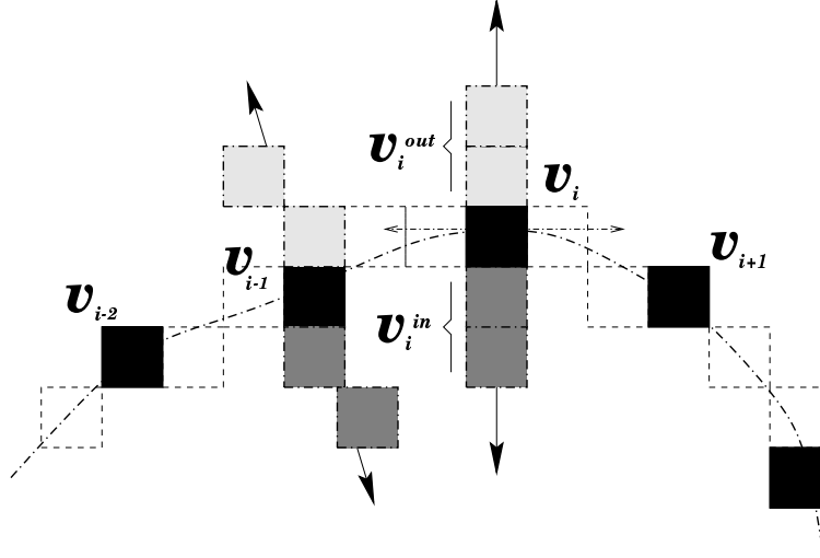
FIG. 1: Portion of a contour model showing five connected nodes and the set of points \mathbf{v}_i^{in} and \mathbf{v}_i^{out} used in the external energy term. N_{in} = N_{out} = 2 in this example.
