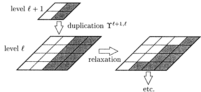
Fig. 6. “Coarse-to-fine” minimization strategy.
