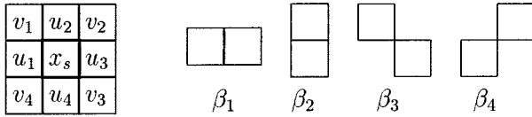
Fig. 1. Second-order neighborhood and associated labeling notations; the four types of two-site cliques and associated parameters in the anisotropic Ising model.
