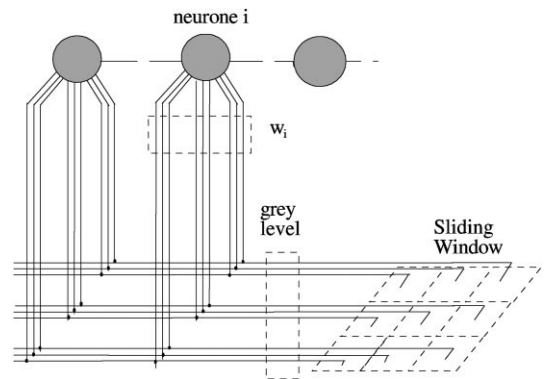
Fig. 4. Model of the SOM used for the segmentation. An 3 \times 3 sliding window is used to feed the SOM.
