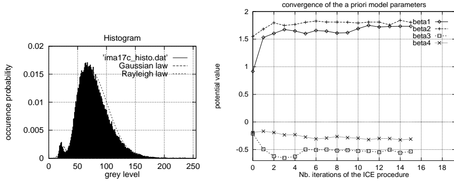
Fig a: Image histogram of the picture reported in Figure 3.a and estimated mixture Fig b: Convergence of the estimation of the a priori parameters
