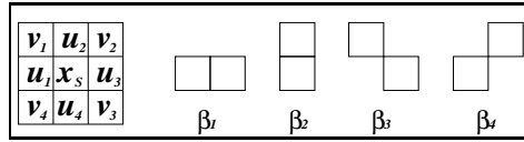
Fig. 1. 2^{nd} order neighborhood and two-site associated cliques.
