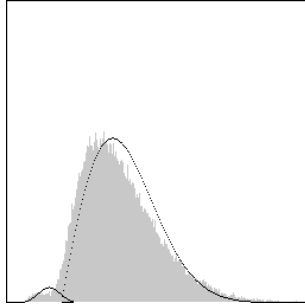
Fig 8.d: Image histogram of the picture reported in Figure 8.a and estimated mixture
