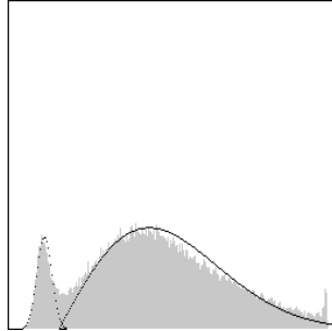
Fig 7.d: Image histogram of the picture reported in Figure 7.a and estimated mixture
