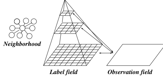
Fig. 5. Neighborhood system and the multiscale relaxation structure.
