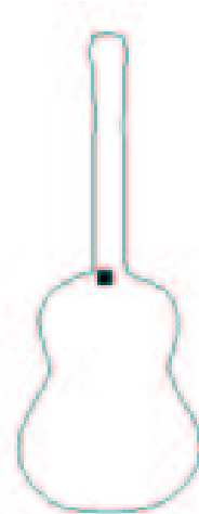
Figure 4: Mean shape and its centroid.
