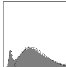
Fig C 0 : Image histogram and estimated mixture (EM)
