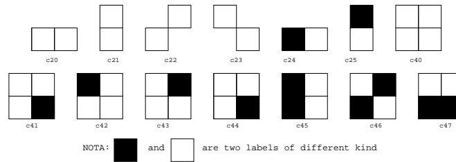
FIG. 2 – Particular configurations c_{ij} of labels on two-site and four-site cliques adopted to express specific geometric shapes. The set of cliques is noted \mathcal{C}
