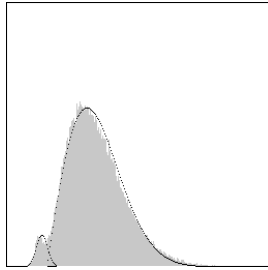
Fig C 0 : Image histogram and estimated mixture (SEM)
