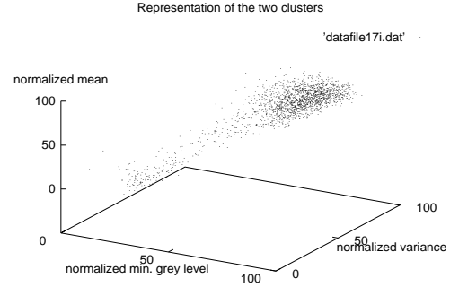
Fig B 1 : representation of the two clusters for k-mean algorithm
