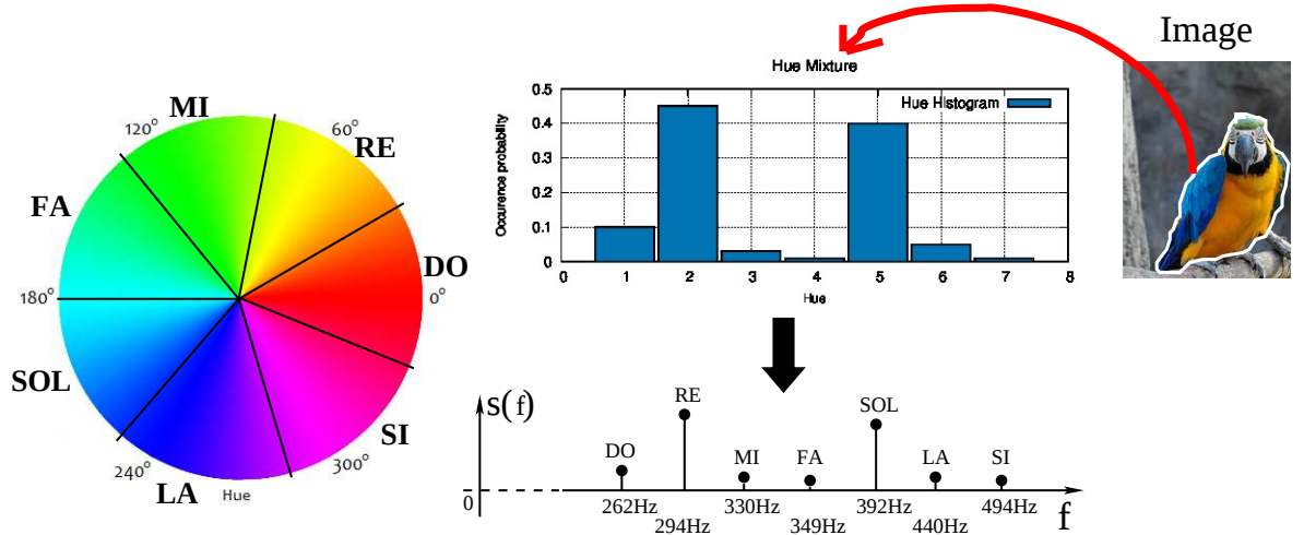
FIGURE 2.2 : Hue Translation : the re-quantized seven-bin hue histogram of each region is first estimated and then converted into an impulse function weighted by the corresponding value of the histogram, in the frequency domain, centered on the frequency corresponding to the different notes of the musical game.
