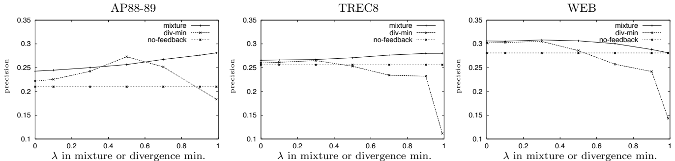
Figure 2: Sensitivity of precision to feedback model parameters on AP88-89 (left), TREC8 (middle), and WEB (right). In each plot, the horizontal line is the non-feedback performance, and the other two lines correspond to the two feedback methods respectively. Note that the x-axis means different \lambda for different methods. For each dataset, the interpolation coefficient was set to \alpha = 0.5 .
