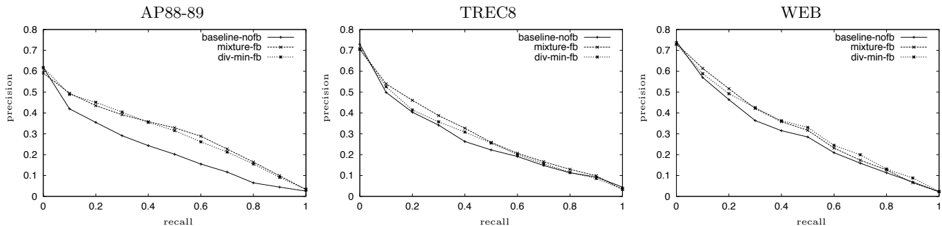
Figure 1: Effect of feedback on AP88-89 (left), TREC8 (middle), and WEB (right). In each plot, the two feedback methods are compared with the baseline simple language modeling approach (no feedback).
