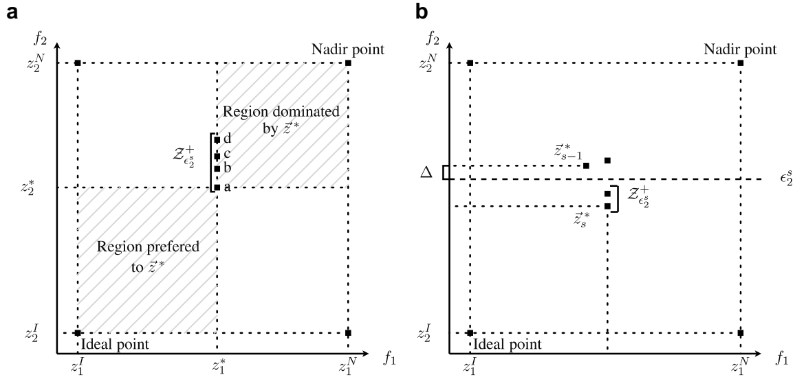
Fig. 1. (a) Illustration of the dominance relation among elements of \mathcal{Z}^+ . (b) Illustration of two consecutive points in the sequence defined by Theorem 3.
