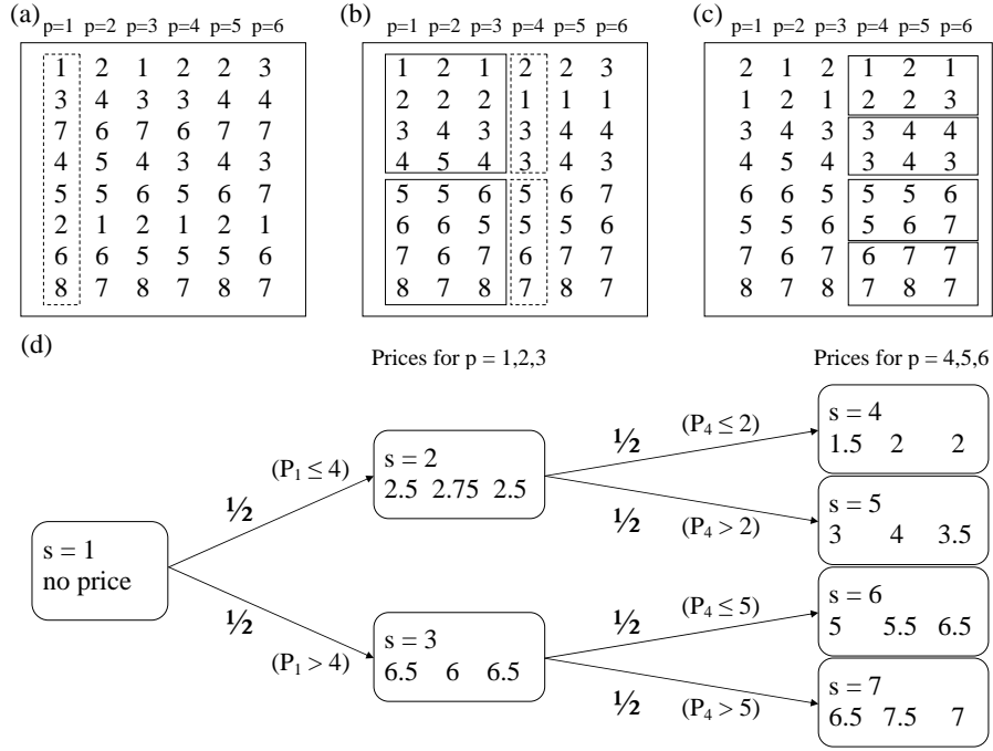
Figure 5: Scenario tree construction example
