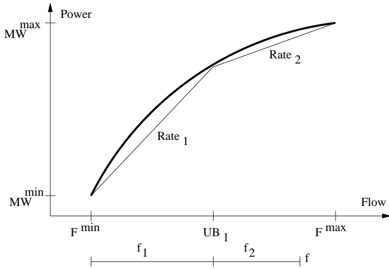
Figure 2: Example of a power generation function at reference head
