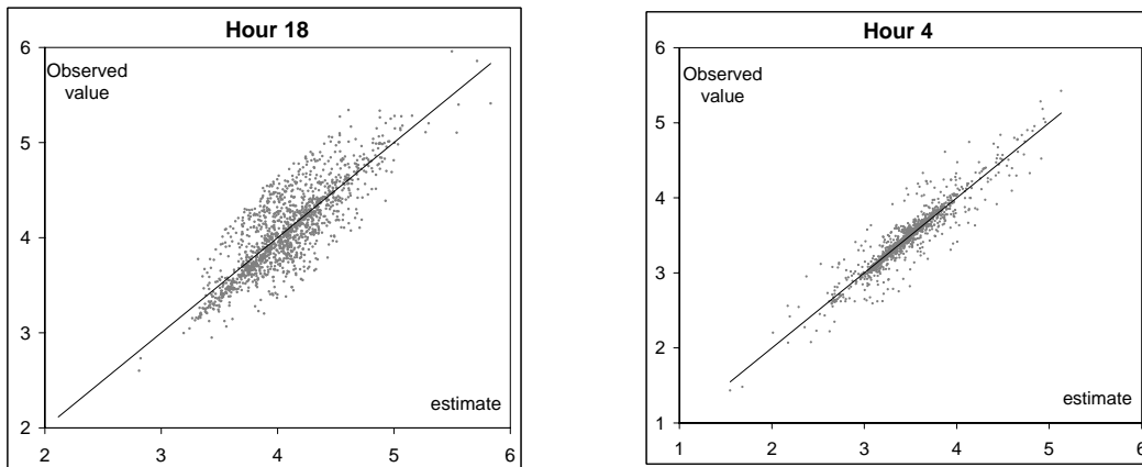
Figure 6: Linear relationship observed in the worst case ( i = 18 , R2_{18} = 0.685 ) and in the best case ( i = 4 , R2_4 = 0.879 )
