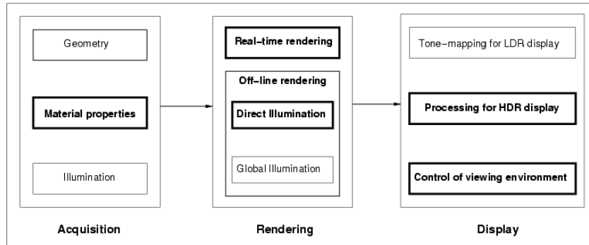
Figure 1.1: Overview of stages of the realistic image synthesis pipeline including acquisition, rendering and display. Individual components of the pipeline that are discussed as part of this dissertation are highlighted.
