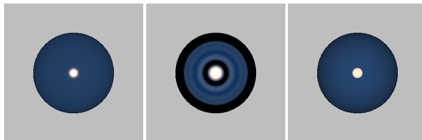
Figure 3.3: An illustration of the suppression of ringing through fitting analytical BRDF models. Left: original acrylic blue paint BRDF. Center: 10^{\text{th}} order zonal reconstruction, rendered after transformation into SH, exhibiting severe ringing artifacts. Right: Corresponding D-BRDF fit to the zonal reconstruction.
