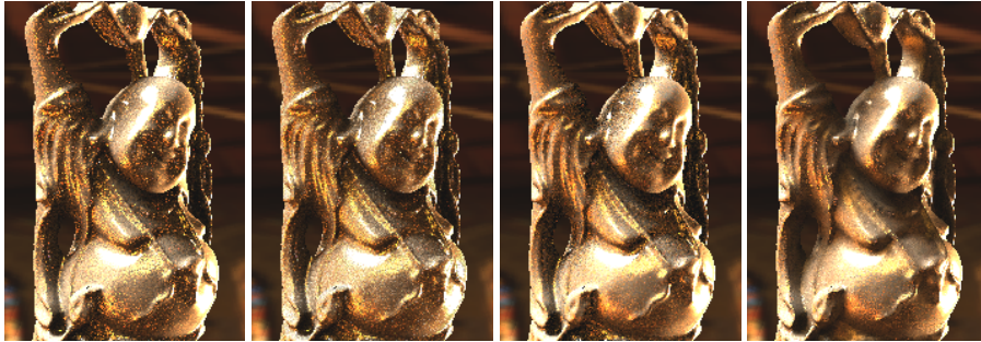
Figure 4.11: Buddha model (Phong BRDF s = 50 , k_s = k_d = 0.5 ) in an indoor HDR EM. Left: Importance sampling from EM, 200 samples/pixel. Center Left: Multiple importance sampling from EM (140 samples/pixel) and BRDF (40 samples/pixel). Center Right: Bidirectional importance sampling, 20 samples/pixel. Right: Correlated visibility sampling, 16 bidirectional samples ( 1^{st} pass) and 16 Metropolis samples per unoccluded sample ( 2^{nd} pass). Rendering times are identical (16 seconds).
