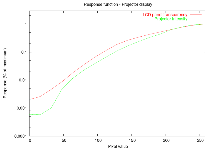
Figure 6.3: Response function of both the LCD panel and the DLP projector in the projector-based display.
