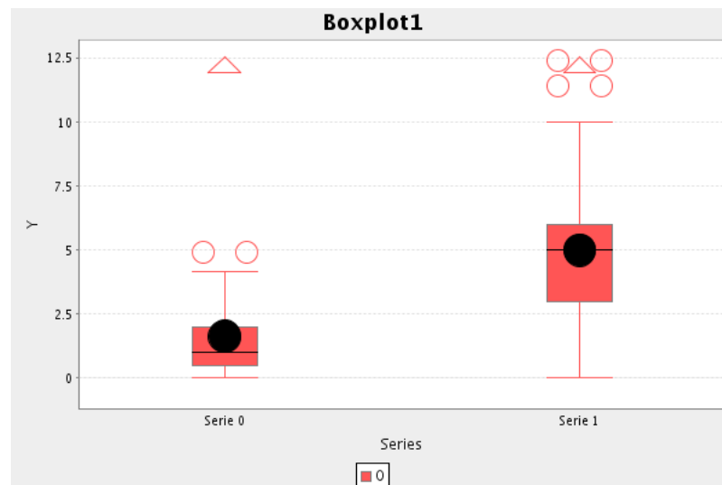
Figure 8: A box-plot
