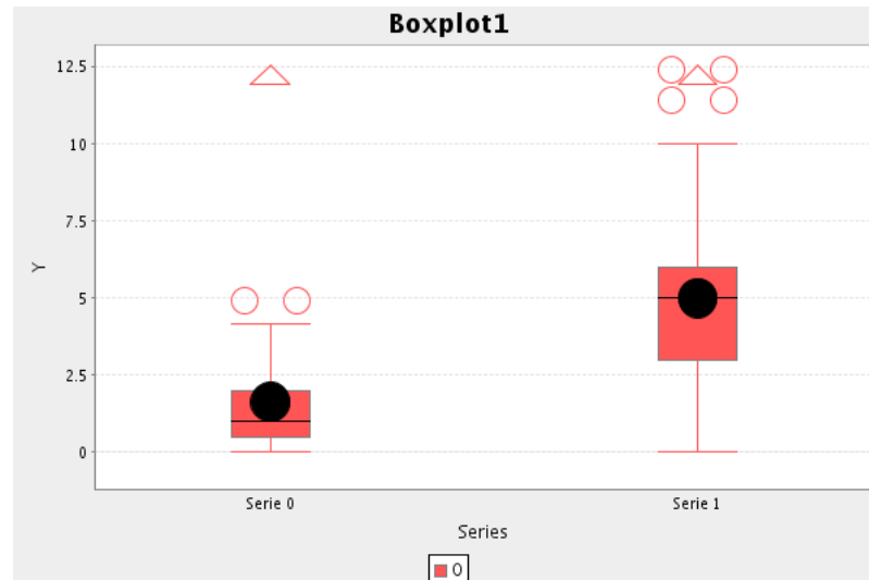
Figure 8: A box-plot
