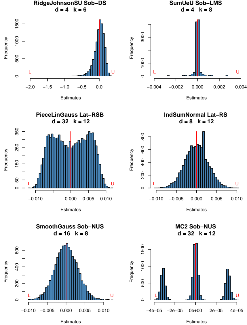
Figure 1: Some histograms of N = 10,000 integral estimates, with k = \log_2(n) . In each case L and U mark the lower and upper extreme sample values and a red vertical line marks the integrand value 0.
