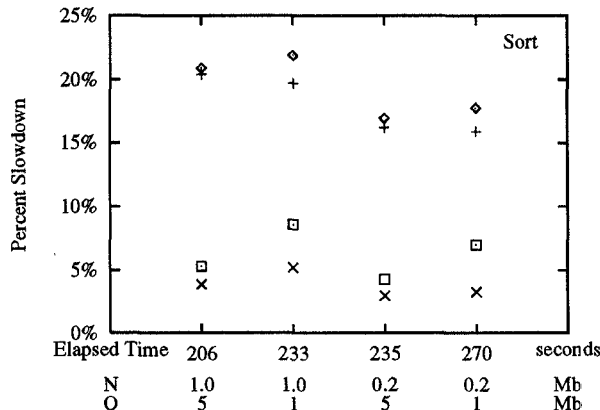
Figure 10: Sort Benchmark: Elapsed Times
