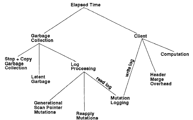
Figure 7: Components of Execution Time
