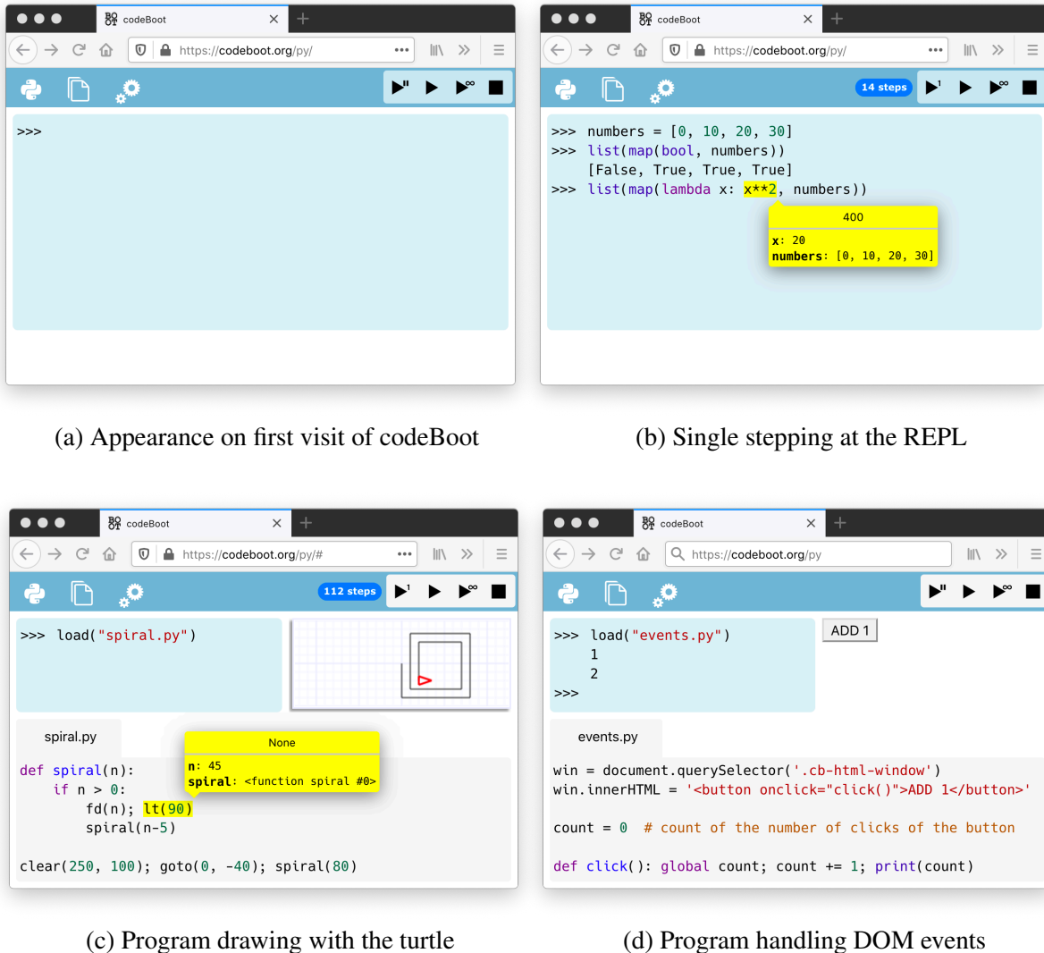
Figure 1: The codeBoot user interface and its features (each screenshot is a clickable hyperlink)
