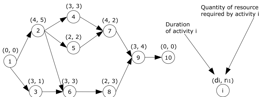
Fig. 1. Example of an (ORD) + (C^f) problem.
