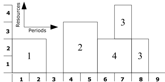
Fig. 7. Example of a better schedule.
