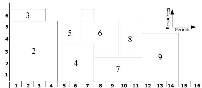
Fig. 9. Example of a schedule induced by an ASL and all its corresponding AL.
