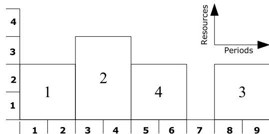
Fig. 6. Schedule resulting from a_1 and a_2 .
