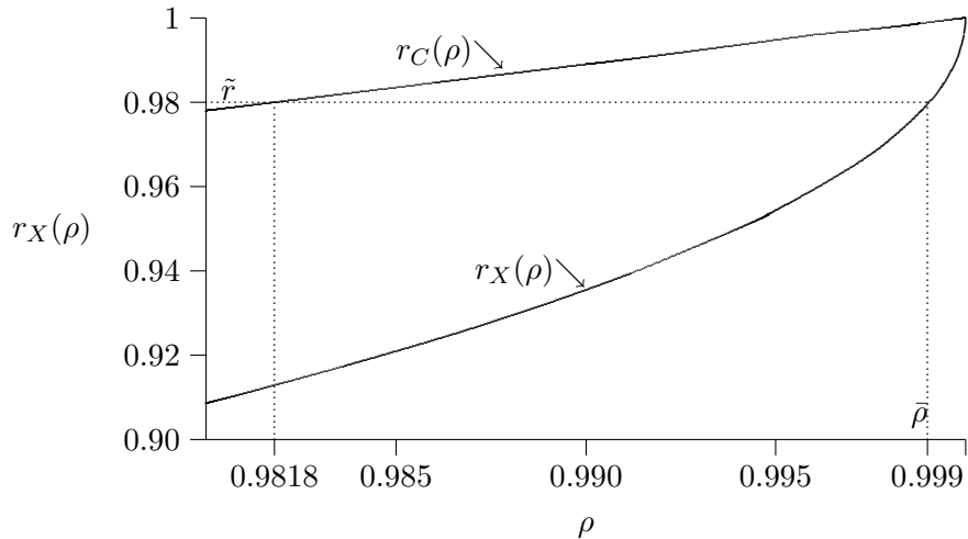
Figure 1: The function r_X(\rho) on [0.98, 1] in the example with binomial marginals with n_1 = 3 ; compared to the function r_C(\rho) given by (6).
