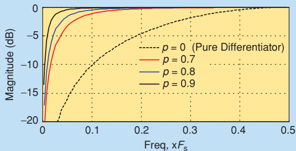
[FIG1] Cascaded differentiator/integrator frequency response.
