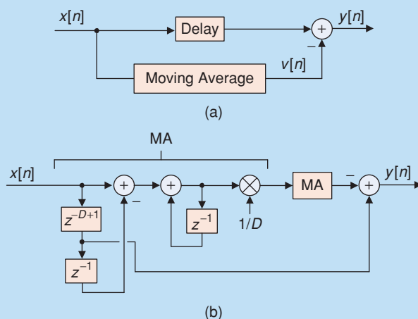
[FIG3] Linear-phase dc blocker: (a) moving average subtraction method and (b) dual-MA implementation.
