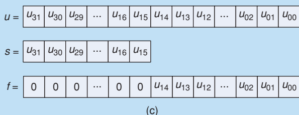
[FIG2] Fixed-point dc blocking filter: (a) simple structure, (b) optimized integrator structure, and (c) bit-wise representation of u , s , and f .
