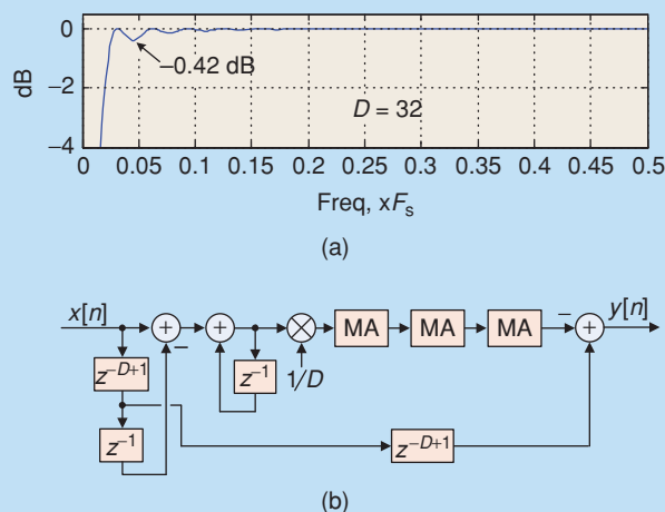
[FIG4] DC blocker: (a) D = 32 dual-MA passband performance and (b) quad-MA implementation.
