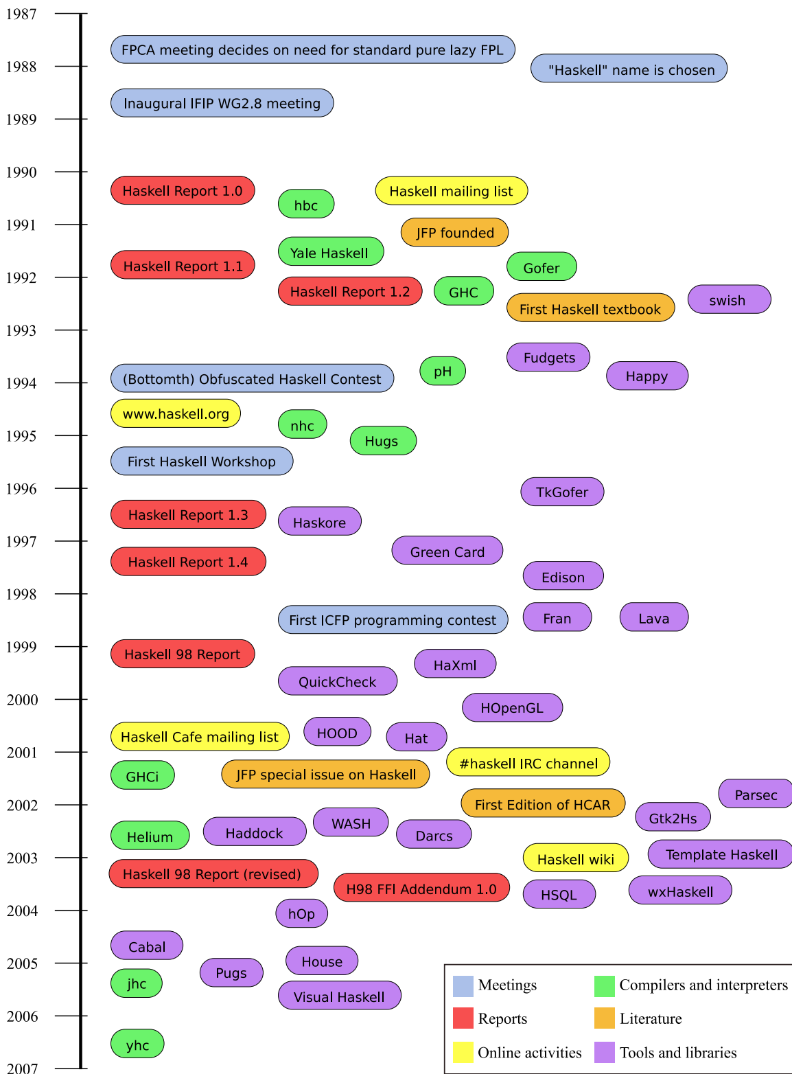
Figure 2. Haskell timeline
