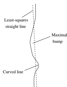
Figure 12: Watt's measure of perceptual curvature
