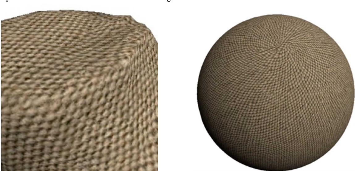
Figure 12: Left: A zoomed-in view of the singular point in the “up” directional field on the Venus model shown in figure 2. Right: A singular point on a sphere.
