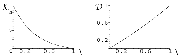
Figure 6. Functionals \mathcal{K} and \mathcal{D} for \rho given by Equation 1 as functions of \lambda for the field of view 90^\circ . Note that when \lambda = 1 , there is no curvature distortion. When \lambda = 0 , then there is no distortion of shape. For a given \mu , we can find \lambda that will approximately minimize the functional \mathcal{F} .
