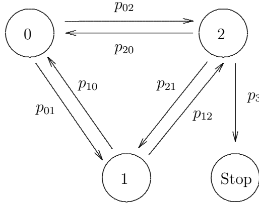
Fig. 1. Evolution of i for our Markov chain.
