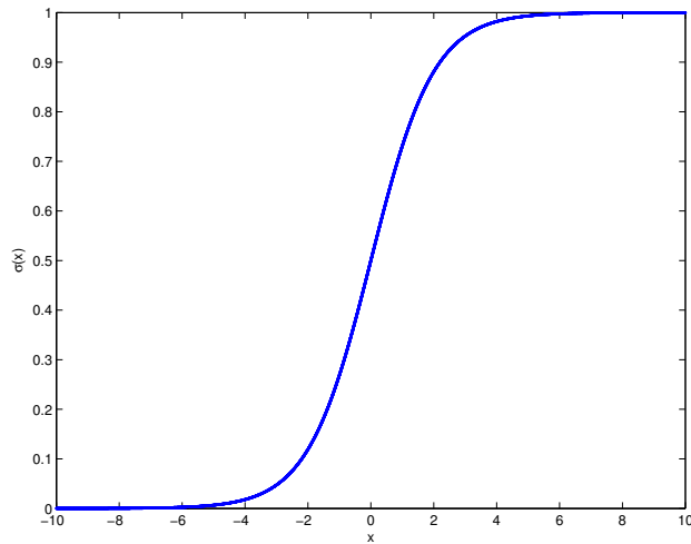
Figure 6.1: Sigmoid function.
